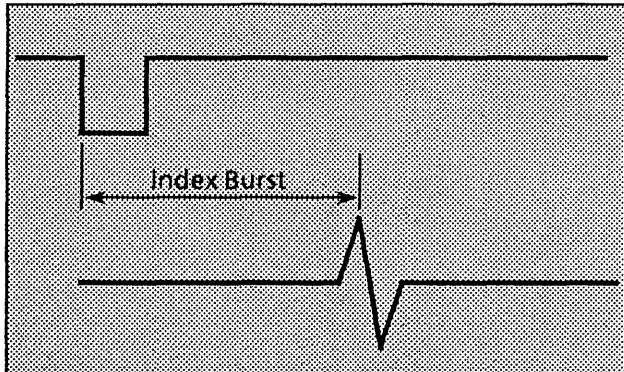
Fig. 9-5 Index Timing
